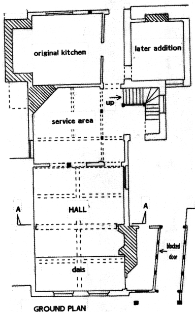
GROUND PLAN
